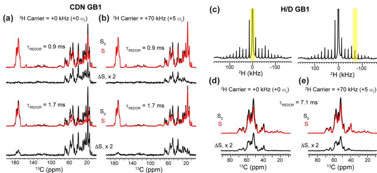
Fig. 3 ^{13}\text{C} - ^2\text{H} REDOR spectra of CDN-GB1 and H/D exchanged GB1. a ^{13}\text{C} REDOR spectra of CDN-GB1 with on-resonance ^2\text{H} REDOR pulses. The ^2\text{H} rf field strength is 20 kHz. The control S_0 , dephased S , and difference \Delta S spectra are shown. b ^{13}\text{C} REDOR spectra of CDN-GB1 with 70 kHz off-resonance ^2\text{H} REDOR pulses. Little dephasing is observed for the sidechain methyl peaks.
