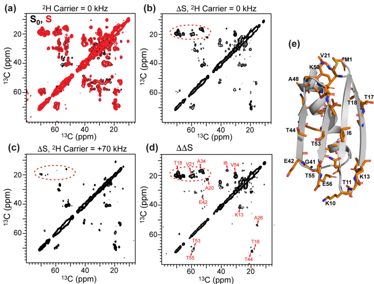
Fig. 4 2D ^{13}\text{C} - ^{13}\text{C} resolved ^{13}\text{C} - ^2\text{H} REDOR spectra of CDN-GB1. The spectra were measured under 14 kHz MAS using a REDOR mixing time of 1.7 ms, and ^2\text{H} and ^{13}\text{C} REDOR rf field strengths of 20 kHz and 50 kHz, respectively. a S_0 (black) and S (red) 2D spectra with on-resonance ^2\text{H} REDOR pulses. Most ^{13}\text{C} signals show similar extents of dipolar dephasing. b \Delta S spectrum obtained from the on-
