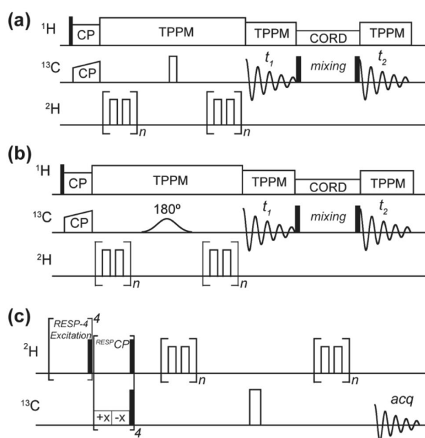
Fig. 1 Pulse sequences for off-resonance ^{13}\text{C} - ^2\text{H} REDOR experiments. a Broadband 2D ^{13}\text{C} - ^{13}\text{C} correlation with ^{13}\text{C} - ^2\text{H} REDOR dephasing. b Ca/Cb-selective 2D ^{13}\text{C} - ^{13}\text{C} correlation with ^{13}\text{C} - ^2\text{H} REDOR dephasing. The 1D variants of the pulse sequences in (a) and (b) acquire the signals during the t_1 period and omit the pulses after that step. c 1D ^{13}\text{C} - ^2\text{H} REDOR with ^2\text{H} - ^{13}\text{C} respiration CP to generate the initial ^{13}\text{C} magnetization. This experiment was applied to perdeuterated bacterial cellulose
