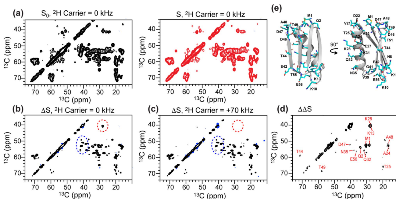
Fig. 5 2D ^{13}\text{C} - ^{13}\text{C} resolved ^{13}\text{C} - ^2\text{H} REDOR spectra of H/D GB1. The spectra were measured with a REDOR mixing time of 7.1 ms under 14 kHz MAS. The rf field strengths of REDOR pulses were 20 kHz for ^2\text{H} and 50 kHz for ^{13}\text{C} . a S_0 (black) and S (red) 2D spectra measured with on-resonance ^2\text{H} REDOR dephasing pulses. b \Delta S spectrum obtained from the on-resonance S_0 and S spectra in (a). c \Delta S spectrum for 70 kHz off-resonance ^2\text{H} REDOR pulses. Note
