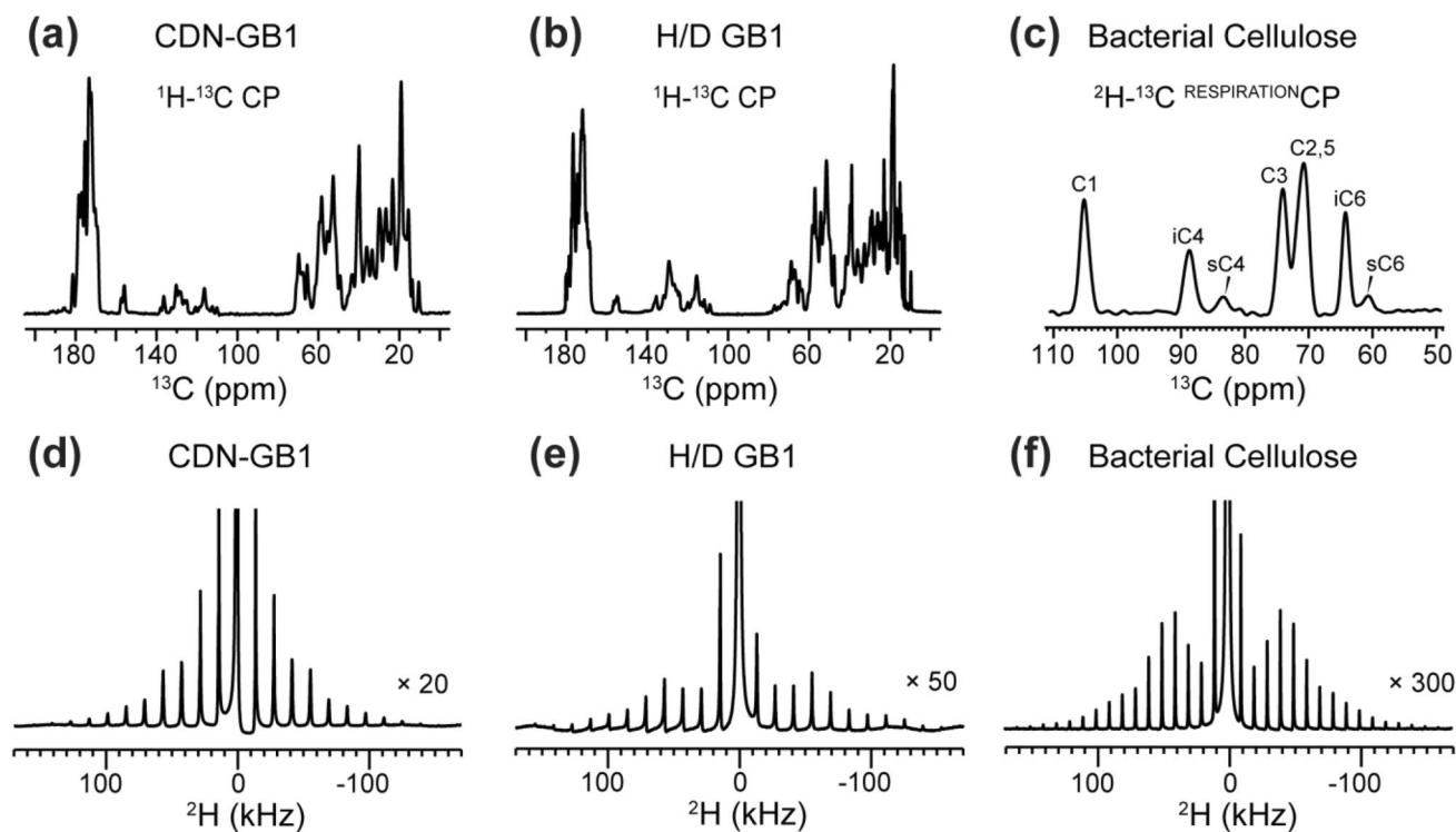
Fig. 2 1D ^{13}\text{C} (a–c) and ^2\text{H} (d–f) MAS spectra of GB1 and bacterial cellulose. a, d CDN-GB1. b, e H/D exchanged ^{13}\text{C} , ^{15}\text{N} -labeled GB1. c, f Perdeuterated bacterial cellulose. All ^2\text{H} MAS spectra were meas-
