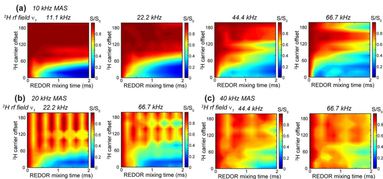
Fig. 8 Numerical simulations of the dependence of ^{13}\text{C} – ^2\text{H} REDOR dephasing on MAS frequency and ^2\text{H} rf field strength ( \nu_1 ). Simulations used the quadrupolar coupling parameters of surface C6 deuterons in bacterial cellulose, with a motionally averaged quadrupolar coupling of 85 kHz and a motionally averaged \eta of 1. a Simulated REDOR dephasing for 10 kHz MAS with ^2\text{H} rf field strengths of 11.1–66.7 kHz. These conditions correspond to 90–15% of each rotation period being occupied by the two ^2\text{H} 180° pulses. The weaker the ^2\text{H} rf field strengths, the more selective the REDOR
