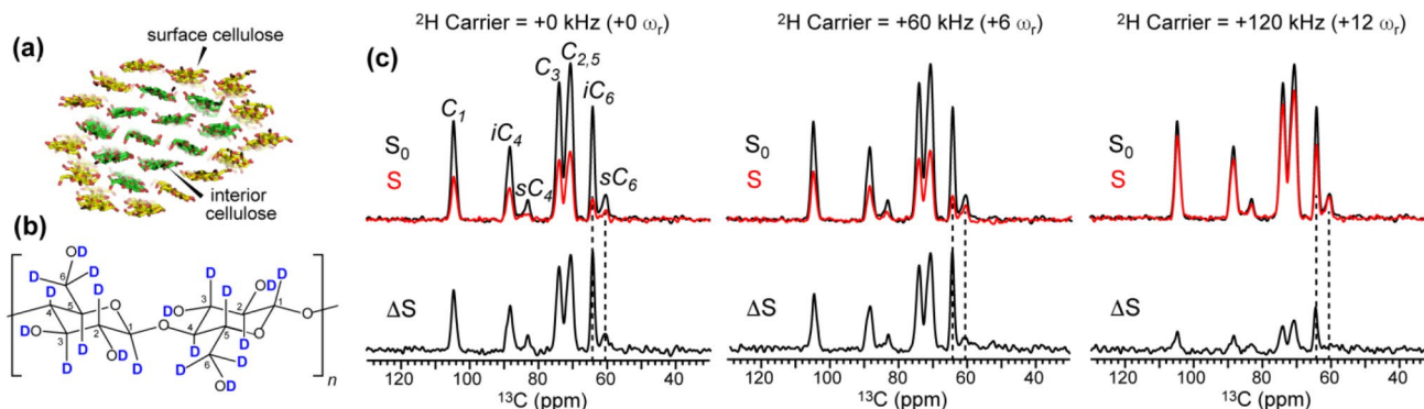
Fig. 6 ^{13}\text{C} - ^2\text{H} REDOR data of perdeuterated bacterial cellulose. a Bacterial cellulose fibrils showing interior cellulose in green and surface cellulose in yellow. b Chemical structure of cellulose. C6 is the only carbon not on the sugar backbone. c 1D ^{13}\text{C} detected and
