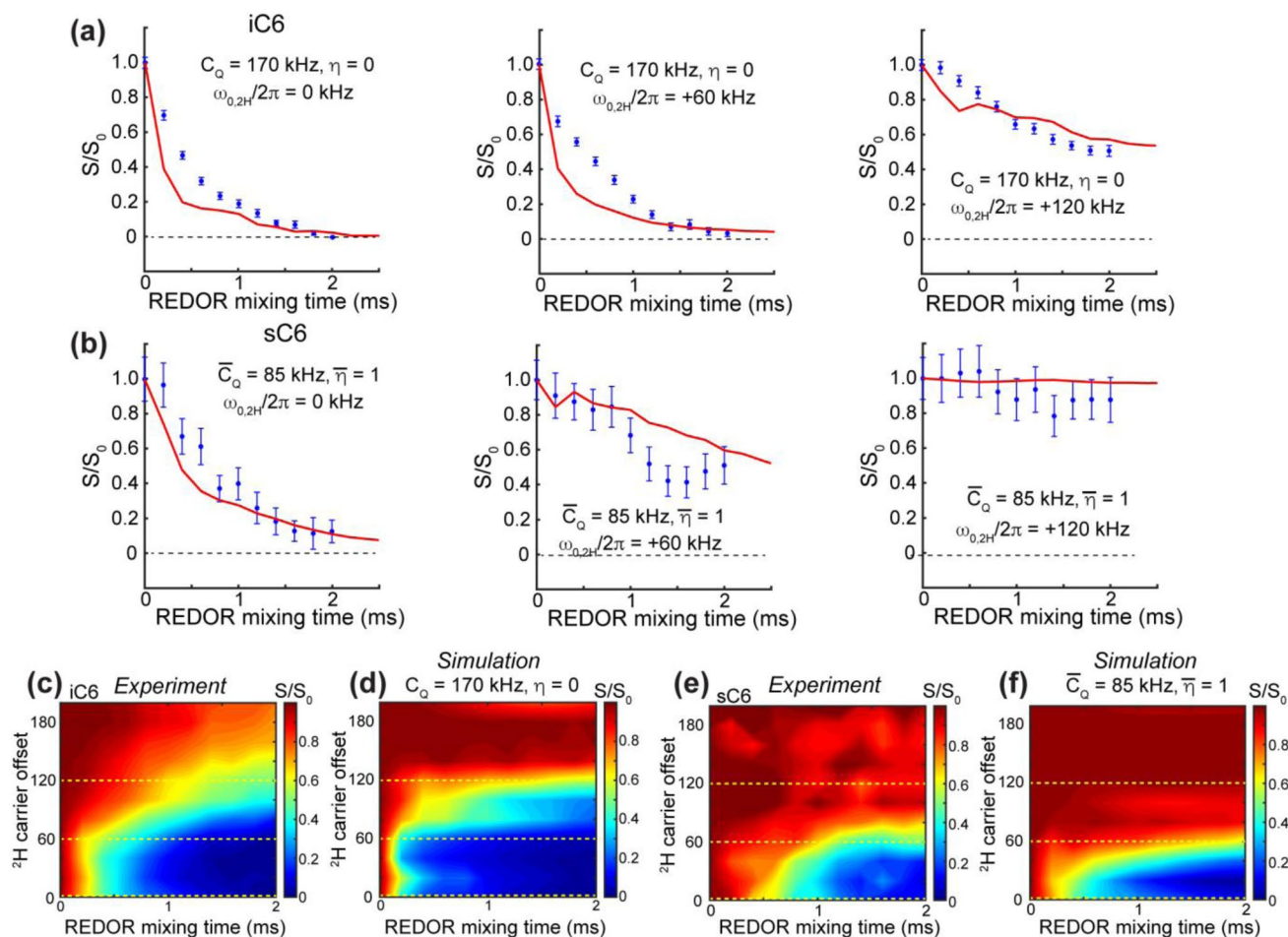
Fig. 7 Numerical simulations of ^{13}\text{C} - ^2\text{H} REDOR dephasing for 10 kHz MAS compared to experimentally measured dephasing for bacterial cellulose. a ^{13}\text{C} - ^2\text{H} REDOR dephasing curves for interior C6, with ^2\text{H} resonance offsets of 0, +60 and +120 kHz, and simulations using a four spin system in which all three ^2\text{H} nuclei have a C_Q of 170 kHz and \eta = 0 . b ^{13}\text{C} - ^2\text{H} REDOR dephasing curves for surface C6, with ^2\text{H} resonance offsets of 0, +60 and +120 kHz, and simulations using a four spin system in which the two ^2\text{H} nuclei bonded to C6 have a motionally averaged C_Q of 85 kHz and a motionally averaged \eta of 1, while the ^2\text{H} nucleus bonded to C5 has a rigid limit C_Q
