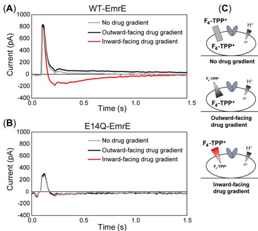
Supplementary Figure 3. Representative solid-supported membrane-based electrophysiology data of F 4 -TPP + transport by EmrE. (A) Current traces for WT-EmrE. (B) Current traces for the transport-dead mutant E14Q-EmrE. (C) Schematic of the TPP + gradients in the different experiments, reproduced from Figure 1 for clarity. At time 0, perfusion of an external buffer set a 2-fold inward-facing H + gradient and a 16-fold F 4 -TPP + gradient (or no gradient) facing the indicated direction. The current trace is at least biphasic for all conditions, with an initial fast positive current (indicating positive charges moving into the liposomes) followed by a slower process with a directionality determined by the gradient conditions. As there is a brief positive spike in the transport-dead E14Q samples, it is likely that some fraction of the positive spike in the WT samples is due to solution exchange artifacts, but this alone cannot account for the much larger spike in the WT samples. In assigning the slow and fast components, we consider several points: 1) It is not uncommon to observe a fast initial signal that represents a non-turnover process, such as substrate binding, and a slower component corresponding to transport 2 . Substrate binding is independent of the transmembrane gradients, and thus should not reverse, which is observed for the fast component. Thus, the initial fast component may represent substrate binding. 2) Substrate-on rates are fast and alternating access of proton-bound EmrE is about an order of magnitude faster than drug-bound EmrE 3 . Furthermore, both substrate-on and alternating access of proton-bound EmrE are essentially independent of drug gradient, and thus should be the same under all conditions. The initial spike is nearly identical under all gradients and it is only the falling edge that varies as the magnitude of the slow component contributes to the signal. Thus, the initial fast component may also represent turnover of proton-bound EmrE, if such turnover is triggered by binding of F 4 -TPP + . 3) The NMR data shows that the alternating-access rate of EmrE bound to F 4 -TPP + is \leq 0.5 \text{ s}^{-1} , and this constrains the rate of net turnover as well. The slow process occurs on the timescale of a second, consistent with this limiting rate for net transport of F 4 -TPP + . Ultimately, while there is not enough data here to definitively determine what processes are represented in the different current phases, the more important parameter is the total transported charge (integrated current), which is shown in Figure 1. The amount and direction of transport is a function of the thermodynamics of the system, and the reversal of the direction of transported charge (note that the slow current switches from positive to negative)
