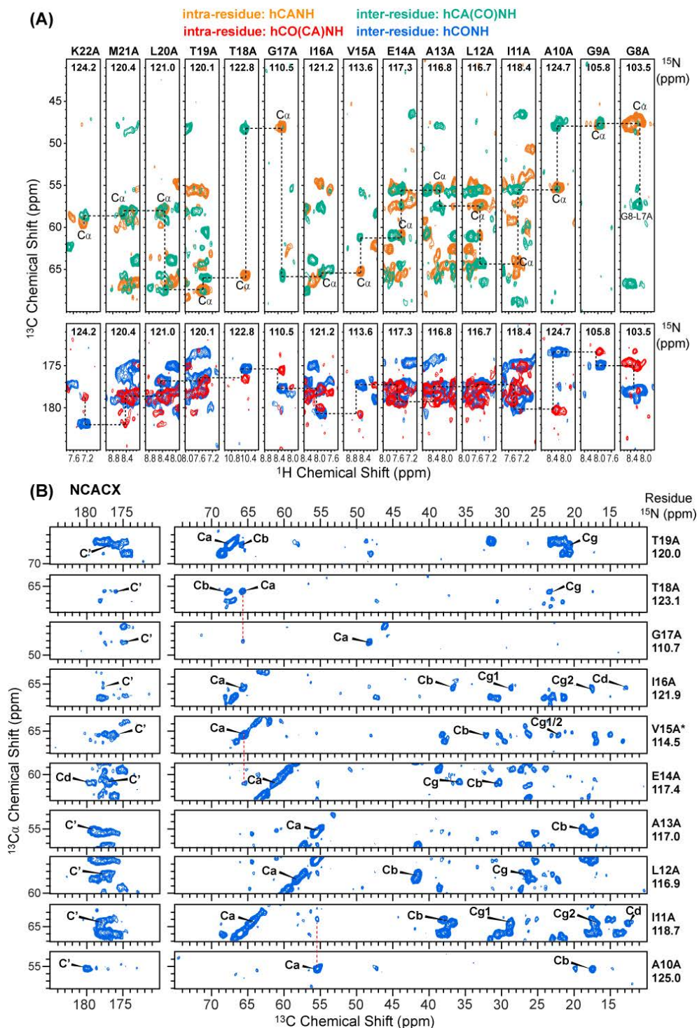
Supplementary Figure 5. Additional 3D spectral strips to illustrate resonance assignment of F_4 -TPP + bound S64V-EmrE in DMPC bilayers. (A) ^1 H-detected spectra for residues G8 to K22 in monomer A. Shown at the top are hCANH and hCA(CO)NH spectra for assigning the C_{\alpha} chemical shifts, and at the bottom are hCO(CA)NH and hCONH spectra for assigning the CO chemical shifts. The spectra were measured under 55 kHz MAS on CDN-labeled protein. (B) Representative strips of the 3D NCACX spectrum for assigning sidechain ^{13} C chemical shifts. The spectrum was measured under 14 kHz MAS using CN-labeled S64V-EmrE.
