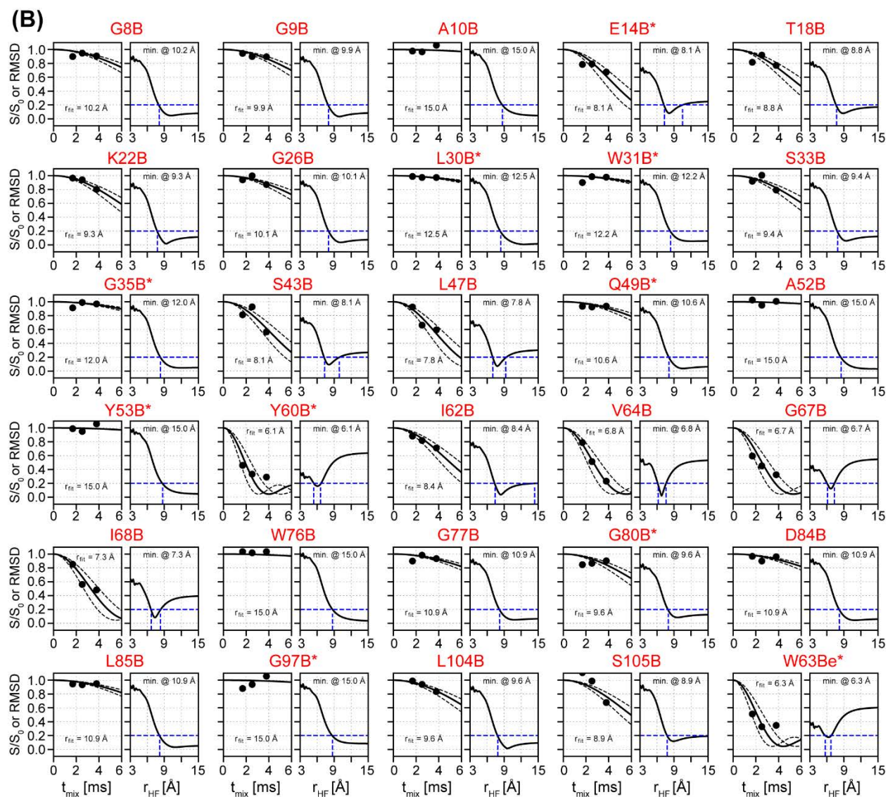
Supplementary Figure 9. Resolved ^1\text{H} - ^{15}\text{N} - ^{19}\text{F} REDOR dephasing curves and RMSDs for extracting best-fit distances. (A) Monomer A data. (B) Monomer B data. For each resolved peak, the REDOR dephasing S/S_0 is plotted on the left and the RMSD between the measured and simulated intensities is shown on the right. Best-fit distance is extracted from the minimum RMSD position, and its simulated REDOR curve is overlaid with the experimental data on the left. Asterisks indicate residues whose signals are partially overlapped in the 2D spectra.
